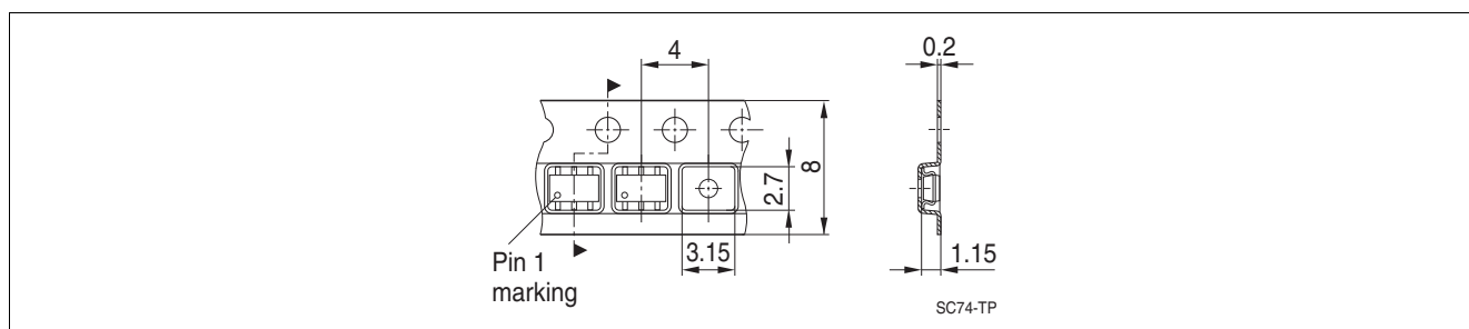
Figure 8 Tape Loading
