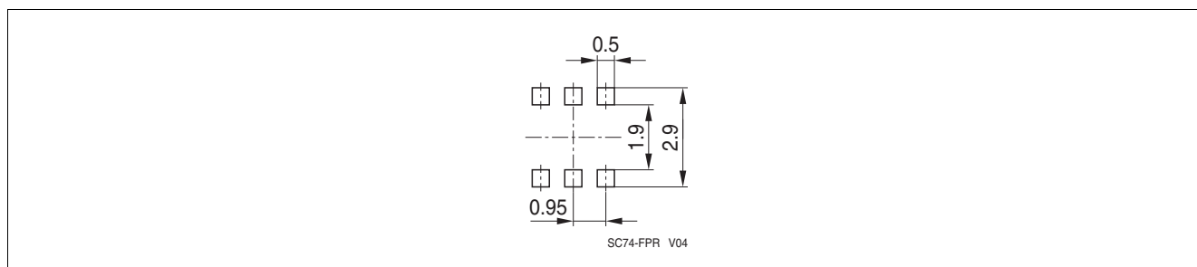
Figure 7 Recommended PCB Footprint for Reflow Soldering
