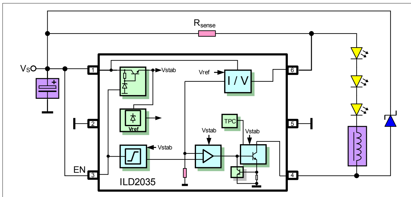
Figure 4 Application Circuit
