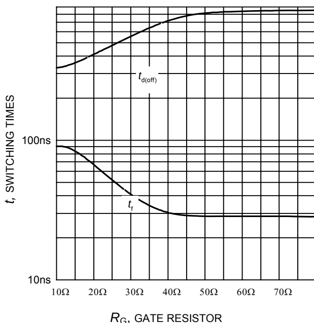
Figure 10. Typical switching times as a function of gate resistor (inductive load, T_J=175^\circ\text{C} , V_{CE}=600\text{V} , V_{GE}=0/15\text{V} , I_C=15\text{A} , Dynamic test circuit in Figure E)
