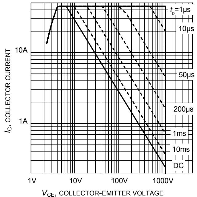
Figure 2. IGBT Safe operating area
