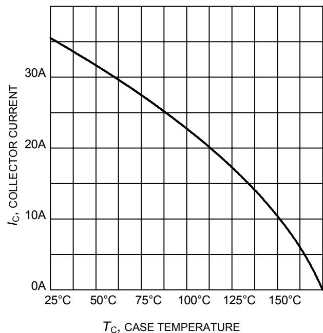
Figure 4. DC Collector current as a function of case temperature
