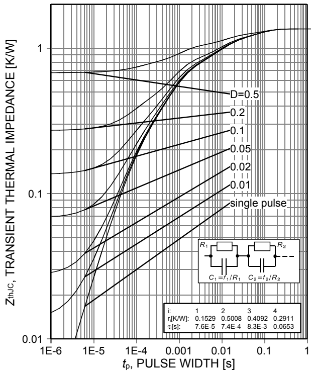
Figure 21. Diode transient thermal impedance ( D = t_p/T )
