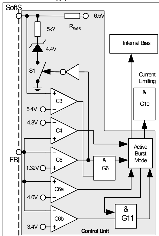
Figure 15 Active Burst Mode
