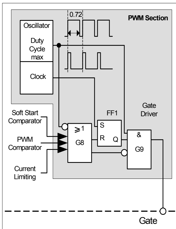
Figure 6 PWM Section
