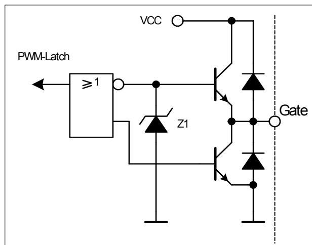
Figure 7 Gate Driver
