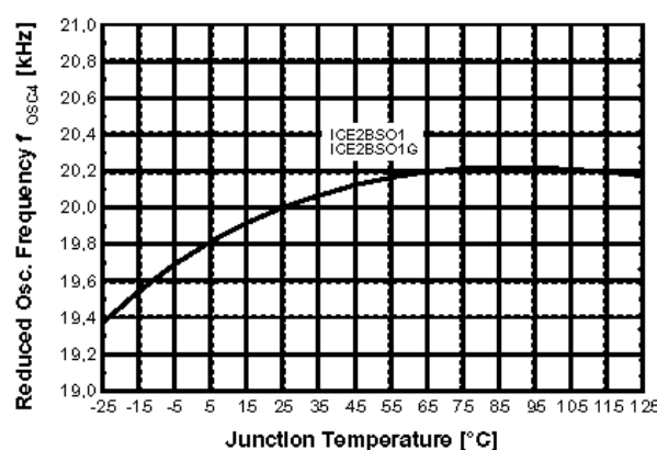
Figure 33 Reduced Osc. Frequency f_{OSC4} vs. T_j
