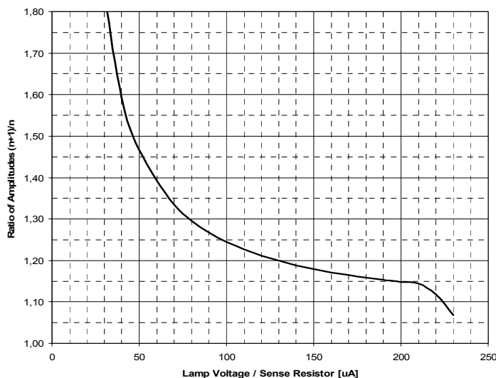
Figure 13 Maximum ratio of amplitudes versus sense current.
