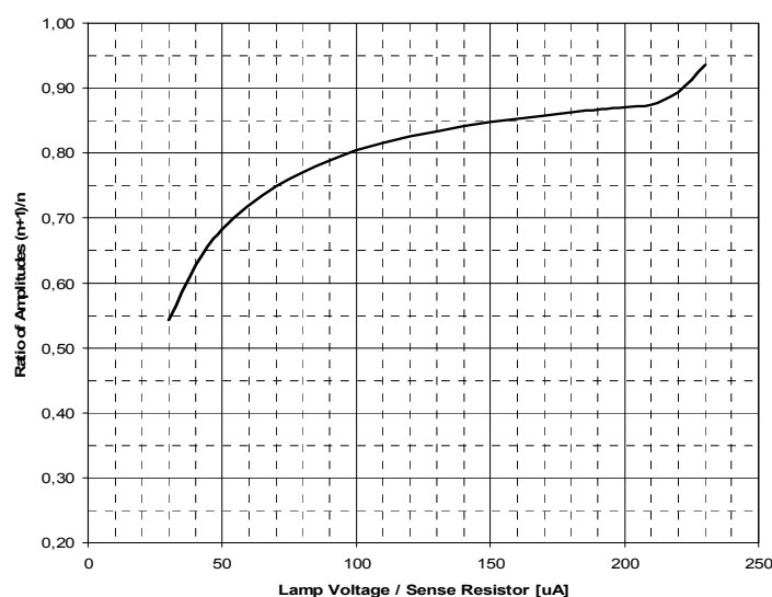
Figure 14 Minimum ratio of amplitudes versus sense current.
