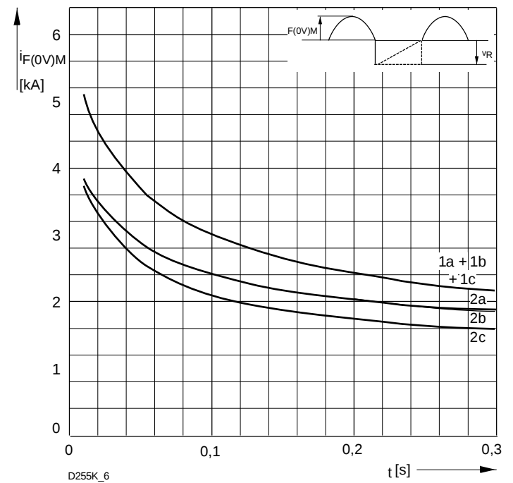
Bild / Fig. 4 Grenzstrom / Maximum overload forward current i_{F(0V)M} = f(t) 1 - I_{FAV(vor)} = 0\text{ A} ; t_{vj} = t_c = 25\text{ °C} 2 - I_{FAV(vor)} = 0\text{ A} ; t_c = 25\text{ °C} ; t_{vj} = 25\text{ °C} a - V_R \leq 50\text{ V} b - V_R = 0,5 V_{RRM} c - V_R = 0,8 V_{RRM}
