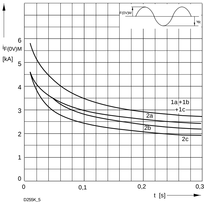
Bild / Fig. 3 Grenzstrom / Maximum overload forward current i_{F(0V)M} = f(t) 1 - I_{FAV(vor)} = 0\text{ A} ; t_{vj} = t_c = 25\text{ °C} 2 - I_{FAV(vor)} = 0\text{ A} ; t_c = 25\text{ °C} ; t_{vj} = 25\text{ °C} a - V_R \leq 50\text{ V} b - V_R = V_{RRM} c - V_R = 0,8 V_{RRM}
