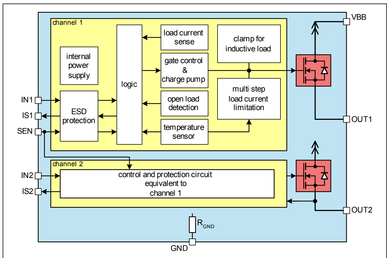
Figure 1 Block Diagram
