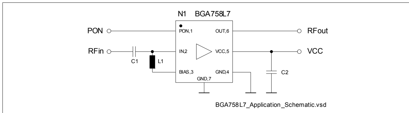
Figure 2 Application Schematic
