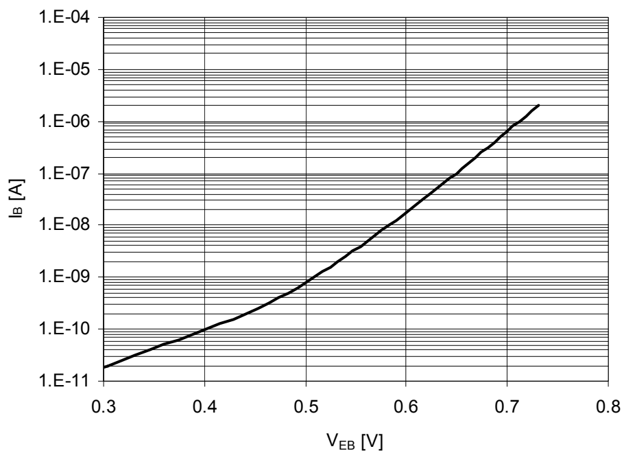
Figure 7 Base Current vs. Base Emitter Reverse Voltage I_B = f(V_{EB}) , V_{CE} = 2 V
