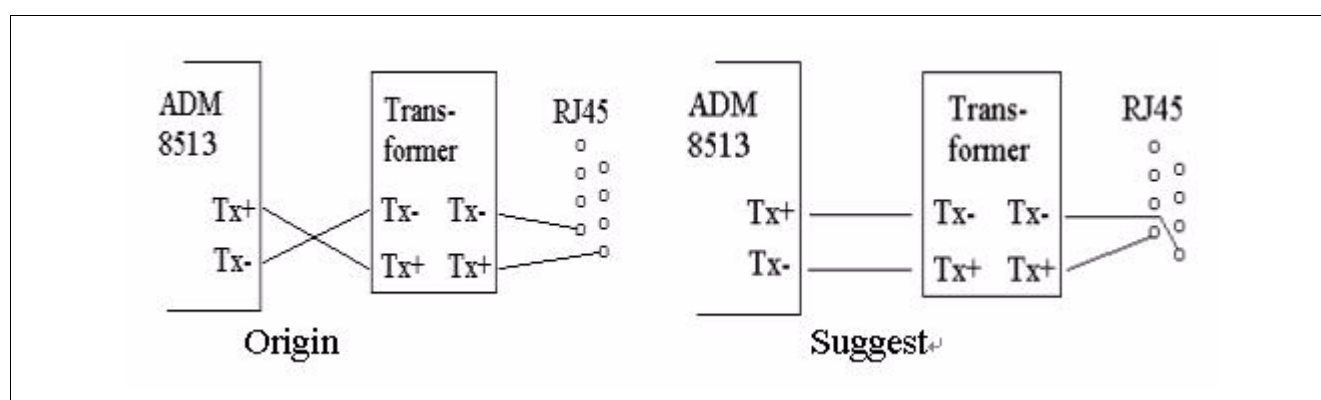
Figure 10 Trace Routing 2
