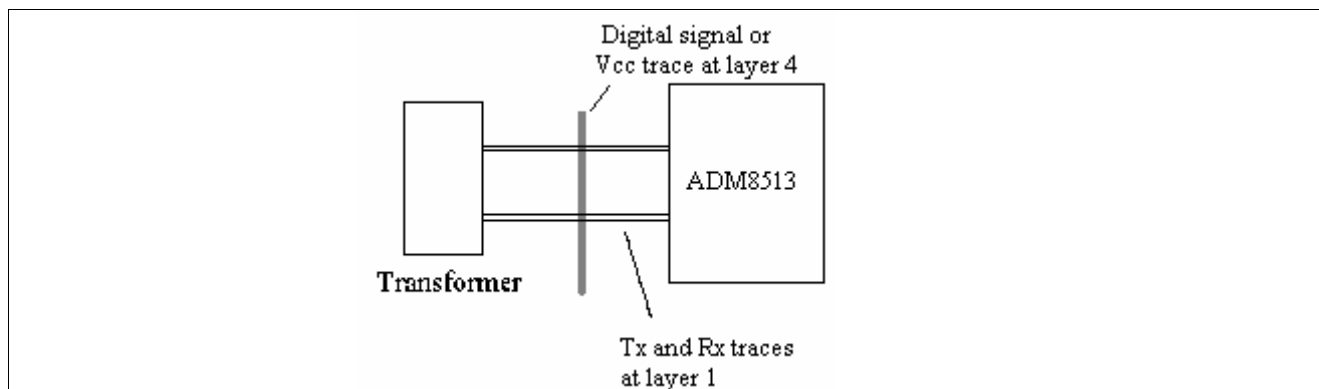
Figure 11 Trace Routing 3
