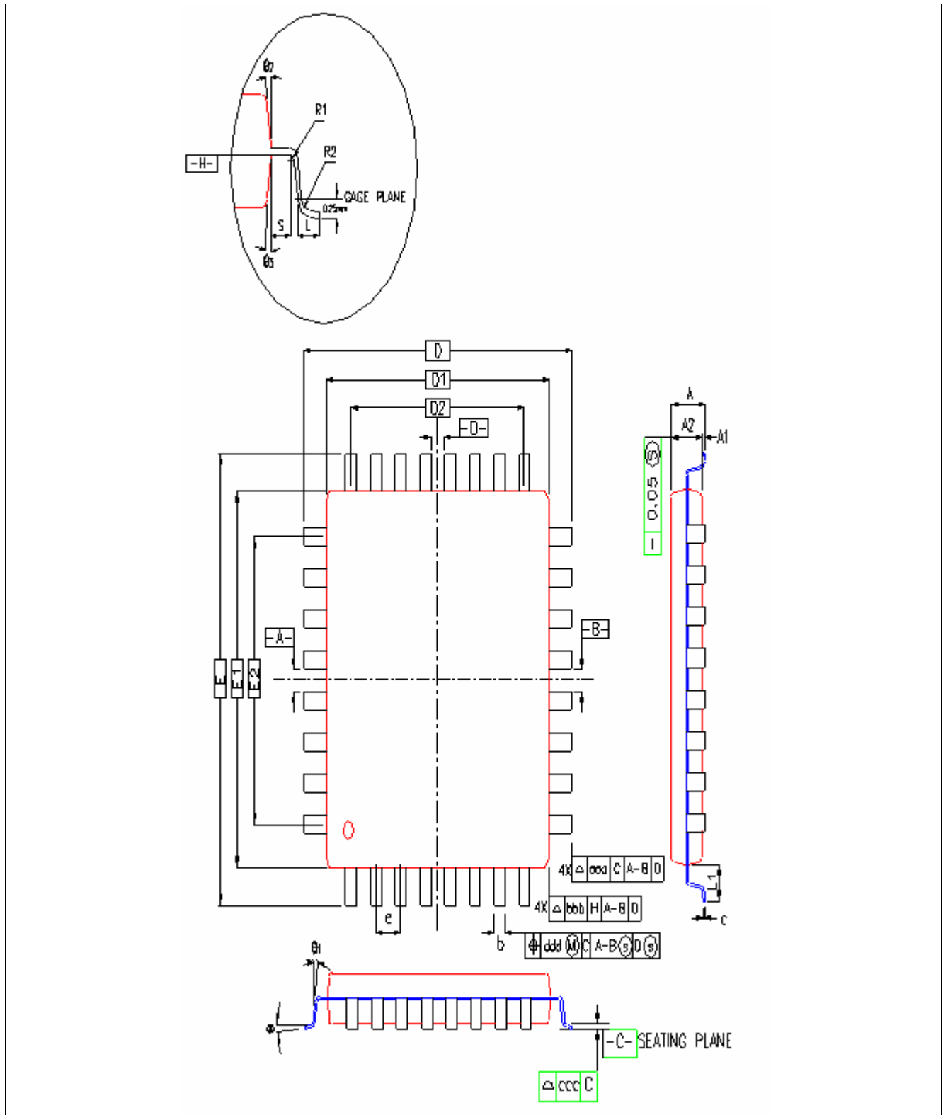
Figure 6 Package
