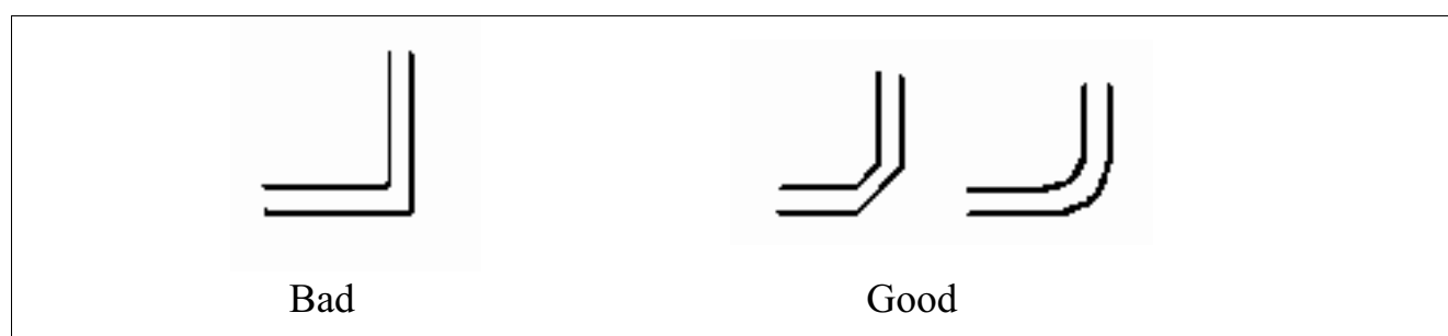
Figure 9 Trace Routing 1
