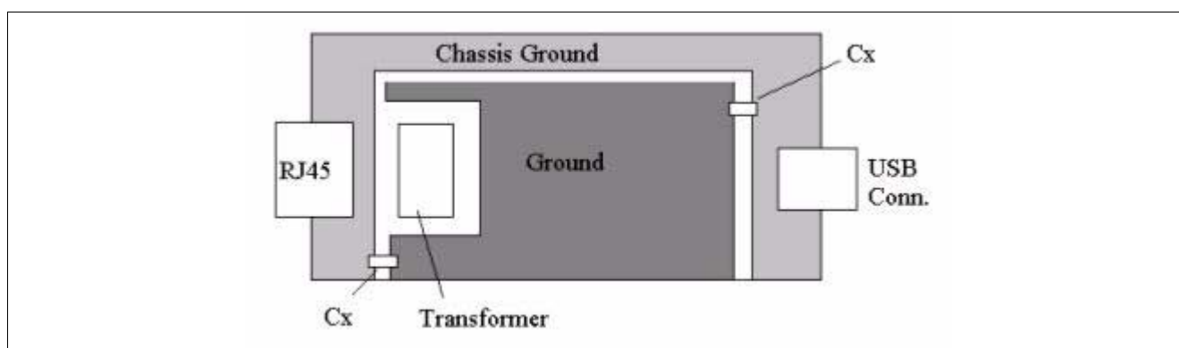
Figure 12 Power and Ground 1
