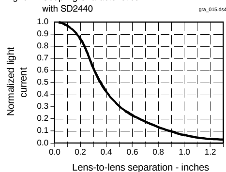
Fig. 6 Coupling Characteristics with SD2440
