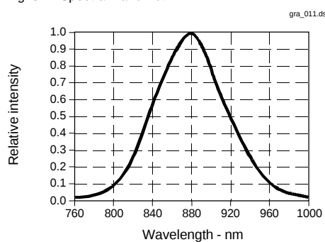
Fig. 5 Spectral Bandwidth
