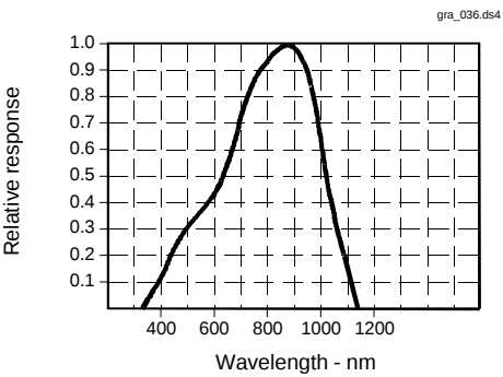
Fig. 5 Spectral Responsivity
