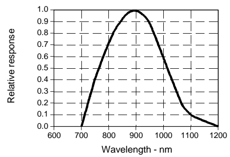
Fig. 5 Spectral Responsivity
