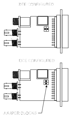
FIGURE 2 - DTE / DCE CONFIGURATION
