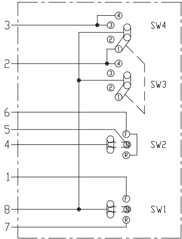
ELECTRICAL SCHEMATIC SHOWN IN NEUTRAL LEGEND
