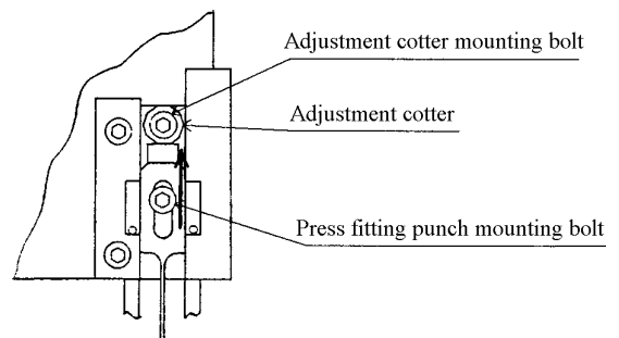
Adjustment cotter
