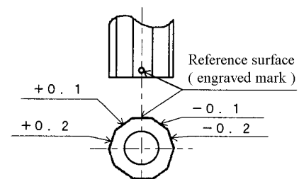
Adjustment cotter
