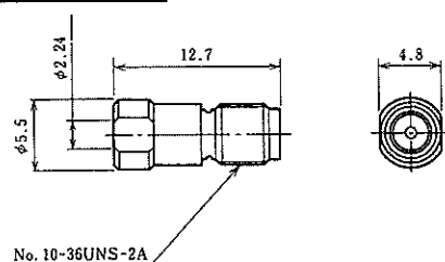
Straight jack
