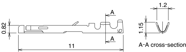
Female contact
