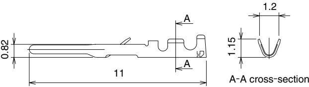
Male contact
