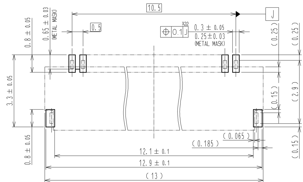
RECOMMENDED PCB MOUNTING PATTERN (No scale) (RECOMMENDED METAL MASK THICKNESS: t=0.1)
