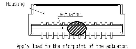
[Actuator operation area(lock and release)] (Top view)
