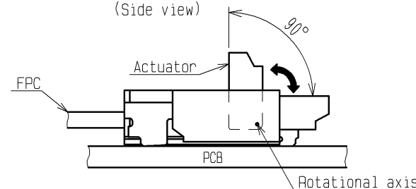
[Actuator movable range] (Side view)
