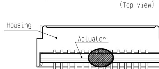
Apply load to the mid-point of the actuator.
