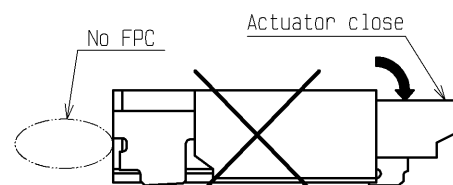
-Improper operation-
