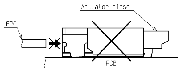
-Improper FPC insertion-
