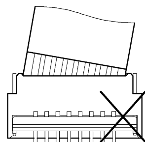
-Improperly assembled- (angle insertion)
