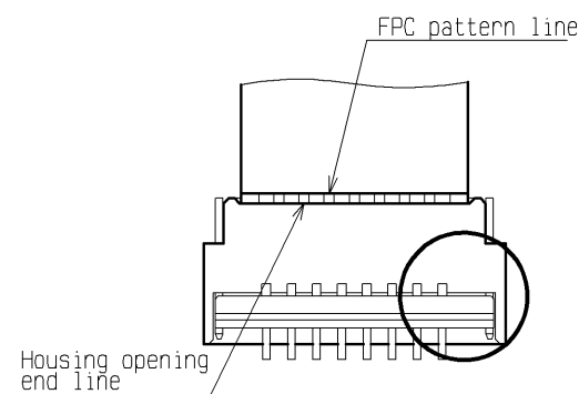
-Properly assembled-
