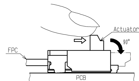
-Proper operation-
