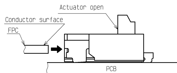
-Proper FPC insertion-
