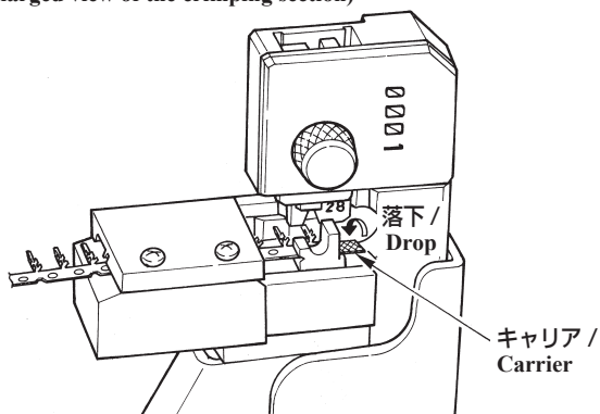
(圧着部拡大図)/ (Enlarged view of the crimping section)
