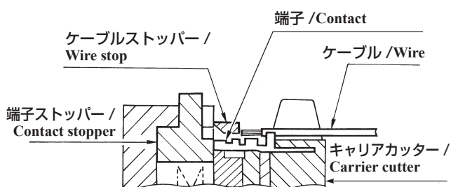
(圧着部拡大図)/ (Enlarged view of the crimping section)
