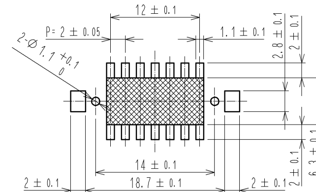
RECOMMENDED PATTERN(2:1)
