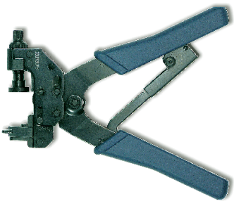
Variokeystone® pressing tool
