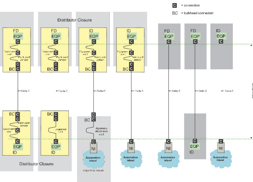
The ISO/IEC 24702 Channel structure
