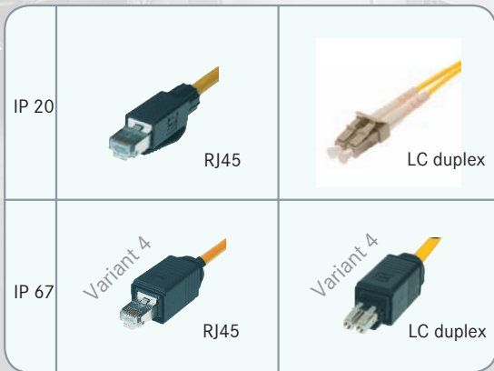
The ISO/IEC 24702 Connectors:
