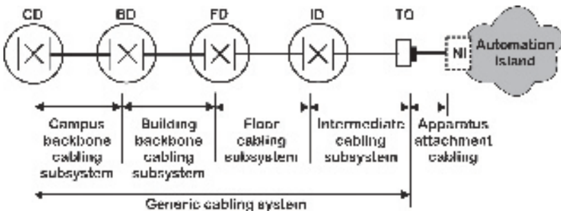
The ISO/IEC 24702 Cabling structure
