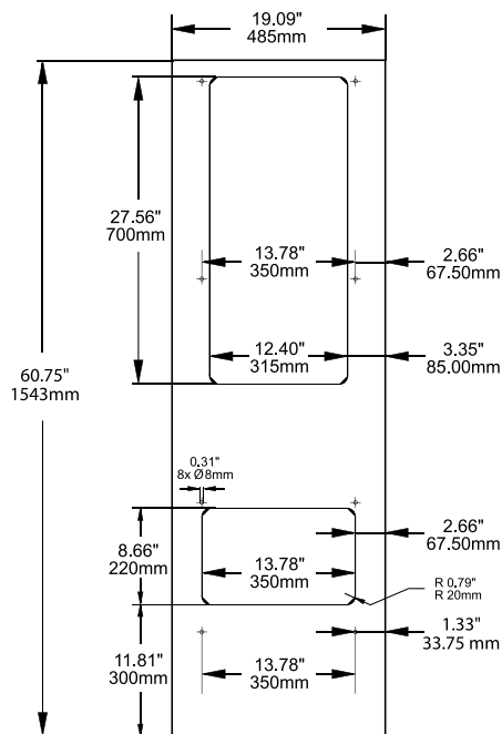
Drilling Template
