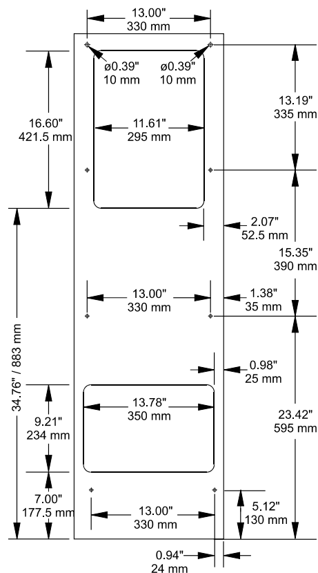
Drilling Template
