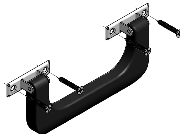
EXPLODED ASSEMBLY VIEW
