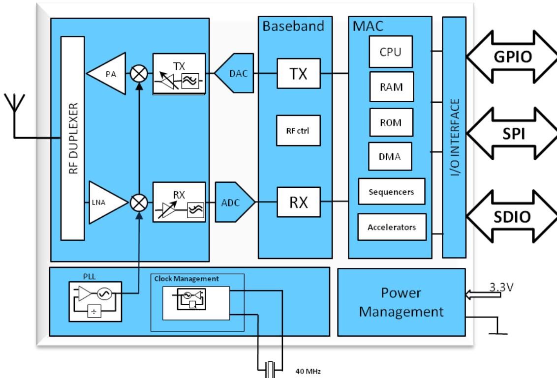
Figure 2.1: Block diagram.
