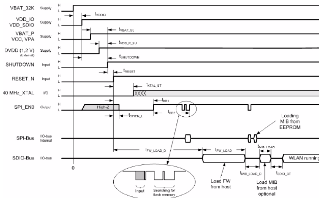
Figure 5-2: Start up sequence with 40 MHz crystal and FW loaded from host via SDIO.
