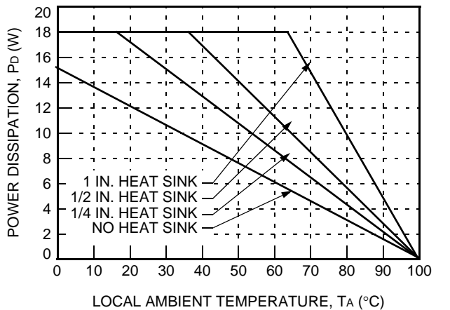
Figure 28. Heat Sink Power Derating Curves; 1.0 m/s (200 lfm); Longitudinal Orientation
