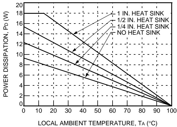
Figure 26. Heat Sink Power Derating Curves; Natural Convection; Longitudinal Orientation
