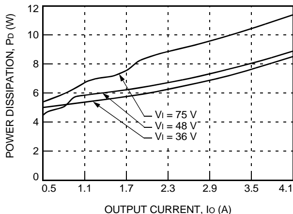
Figure 20. QW050B1 Power Dissipation vs. Output Current at 25 °C
