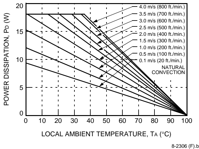
Figure 22. Forced Convection Power Derating with No Heat Sink; Either Orientation
