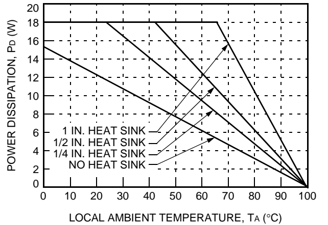
Figure 27. Heat Sink Power Derating Curves; 1.0 m/s (200 lfm); Transverse Orientation
