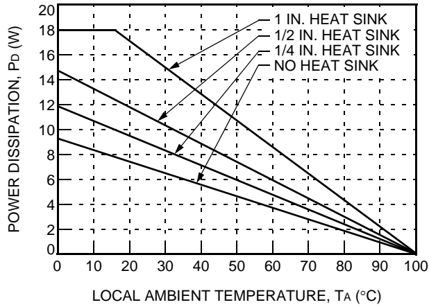
Figure 25. Heat Sink Power Derating Curves; Natural Convection; Transverse Orientation
