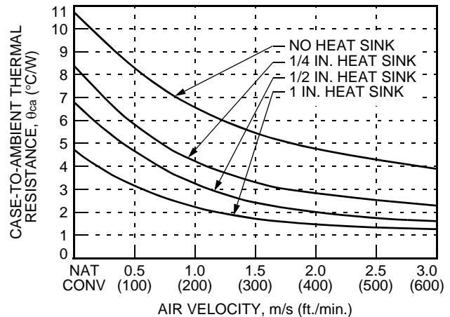
Figure 23. Case-to-Ambient Thermal Resistance Curves; Transverse Orientation
