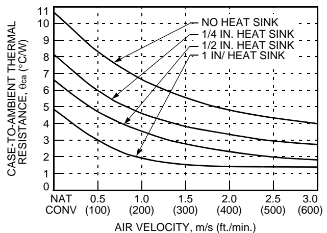
Figure 24. Case-to-Ambient Thermal Resistance Curves; Longitudinal Orientation
