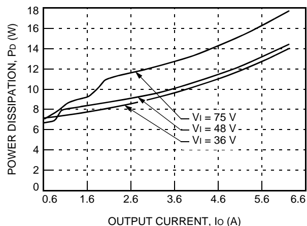
Figure 21. QW075B1 Power Dissipation vs. Output Current at 25 °C
