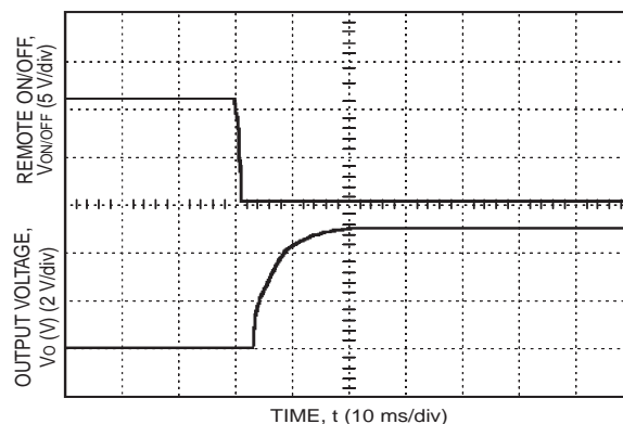
Figure 36. Start-up from Remote On/Off ( I_O = I_{O, \text{max}} ).
