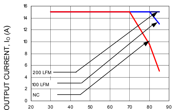
LOCAL AMBIENT TEMPERATURE, T_A (°C) Figure 3. Derating curves for QW015A0F1-H ( V_o = 3.3V ) in transverse orientation ( V_{in} = 48Vdc )
