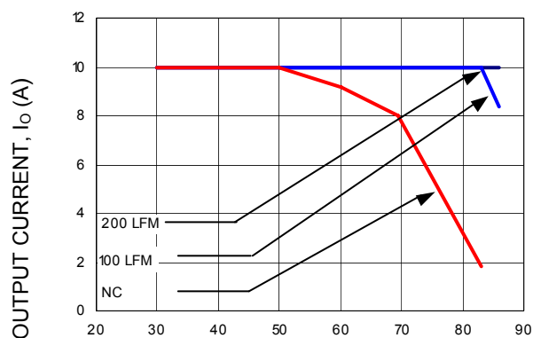
LOCAL AMBIENT TEMPERATURE, T_A (°C) Figure 2. Derating curves for QW010A0A1-H ( V_o = 5.0 ) in transverse orientation ( V_{in} = 48Vdc )
