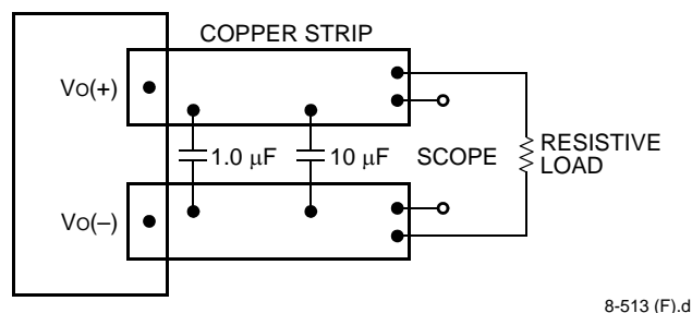
Figure 17. Output Reflected-Ripple Test Setup
