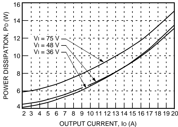
Figure 29. QHW100A1-Q Power Dissipation vs. Output Current at 25 °C
