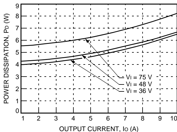
Figure 27. QHW050A1-Q Power Dissipation vs. Output Current at 25 °C
