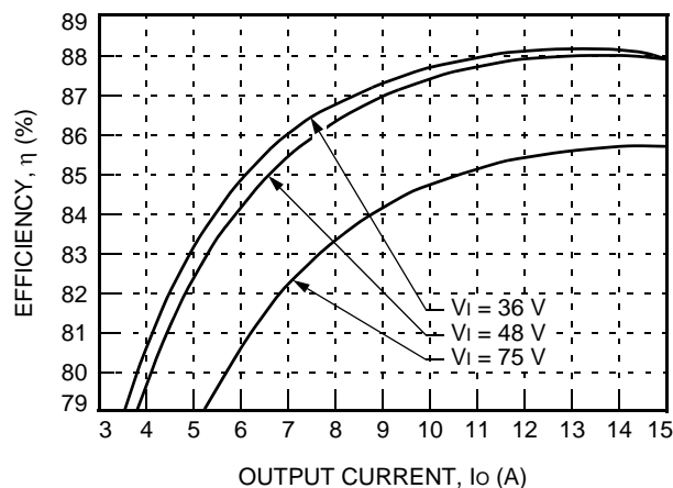
Figure 5. Typical QHW075A1-Q Converter Efficiency vs. Output Current at Room Temperature
