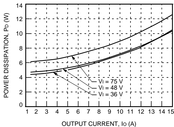
Figure 28. QHW075A1-Q Power Dissipation vs. Output Current at 25 °C
