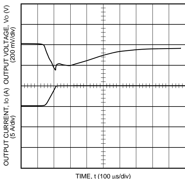
Figure 11. Typical QHW075A1-Q Transient Response to Step Increase in Load from 50% to 75% of I_{O, \max} at Room Temperature and 54 Vdc Input (Waveform Averaged to Eliminate Ripple Component.)
