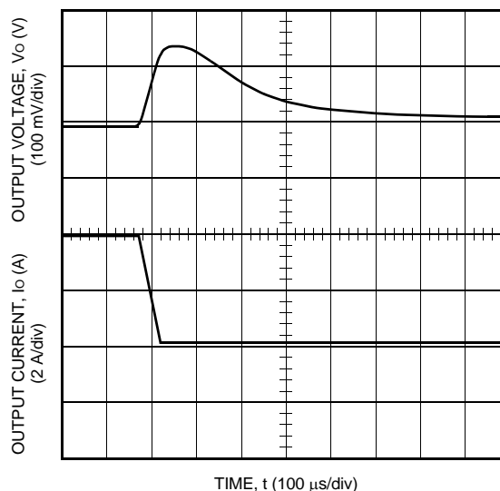
Figure 13. Typical QHW050A1-Q Transient Response to Step Decrease in Load from 50% to 25% of I_{O, \max} at Room Temperature and 48 Vdc Input (Waveform Averaged to Eliminate Ripple Component.)
