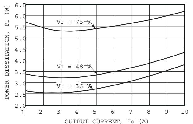
Figure 27. QHW050Y1 Power Dissipation vs. Output Current at 25 °C
