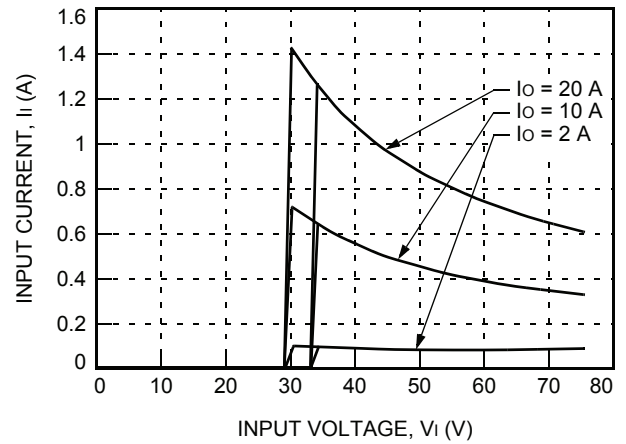
Figure 3. Typical QHW100Y1 Input Characteristics at Room Temperature
