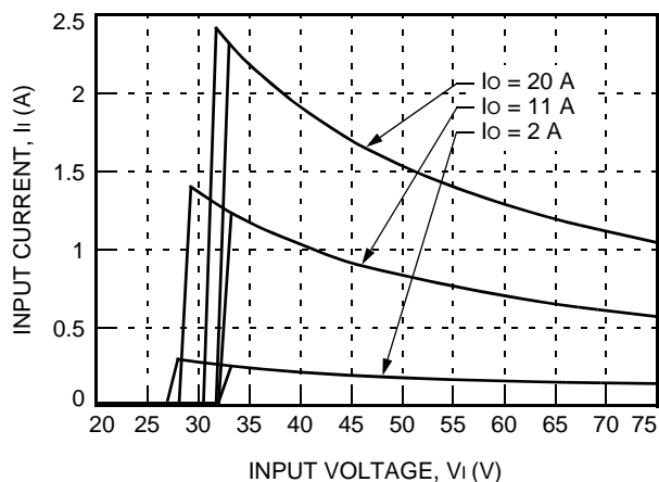
Figure 3. Typical QHW100F1-Q Input Characteristics at Room Temperature
