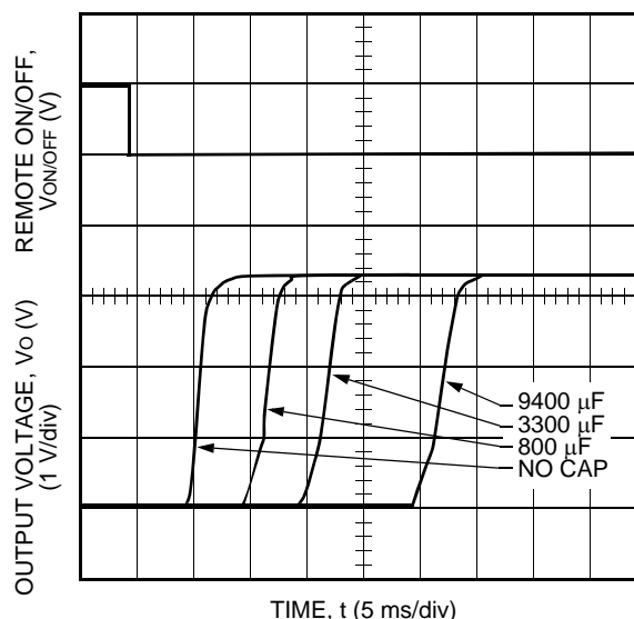
Figure 16. Typical Start-Up from Remote On/Off; I_o = I_{o, \max}
