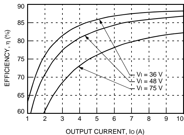
Figure 4. Typical QHW050F1-Q Converter Efficiency vs. Output Current at Room Temperature
