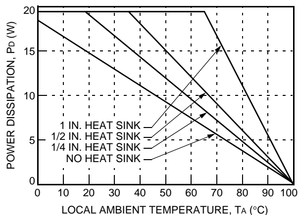
Figure 34. Heat Sink Power Derating Curves; 1.0 m/s (200 lfm); Transverse Orientation
