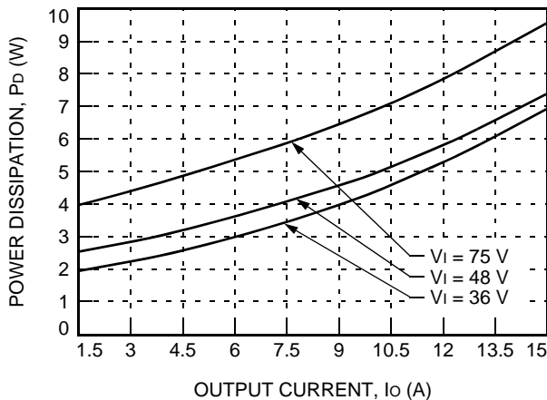
Figure 28. QHW075F1-Q Power Dissipation vs. Output Current at 25 °C
