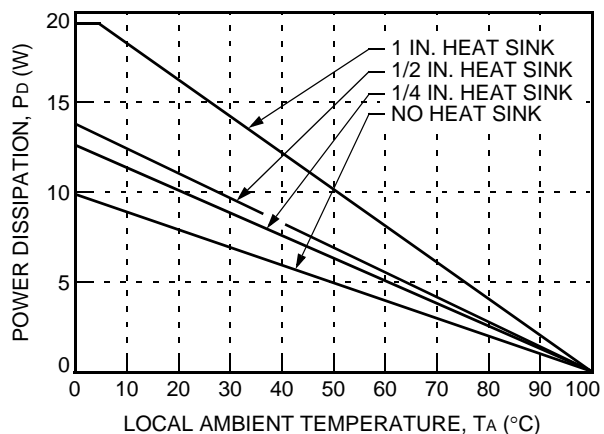
Figure 32. Heat Sink Power Derating Curves; Natural Convection; Transverse Orientation
