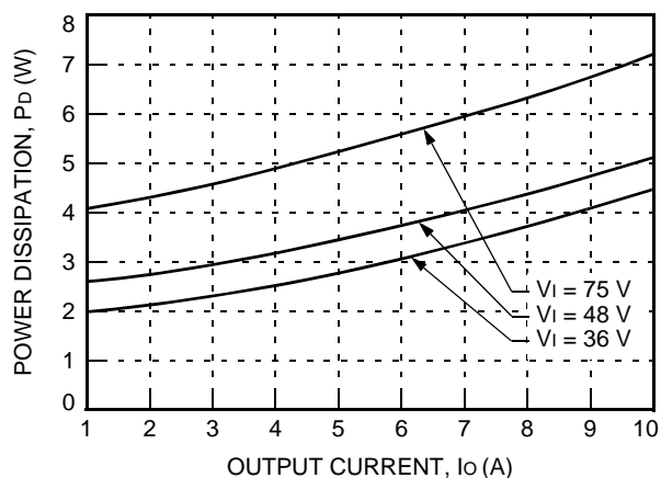
Figure 27. QHW050F1-Q Power Dissipation vs. Output Current at 25 °C
