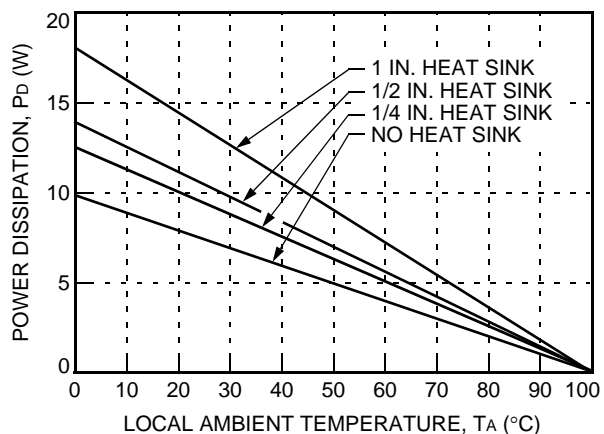
Figure 33. Heat Sink Power Derating Curves; Natural Convection; Longitudinal Orientation
