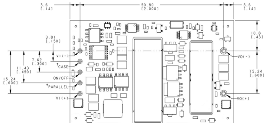
BOTTOM VIEW
