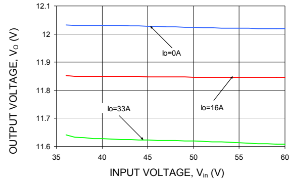
Figure 7. Typical Output voltage regulation vs. Input voltage at Room Temperature.
