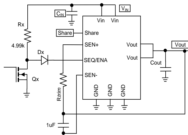
Figure 24. Application Schematic
