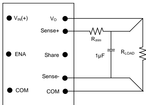
Figure 27. Circuit Configuration for Programming
