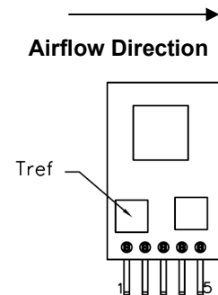
Figure 54. T_{ref} Temperature measurement location.
