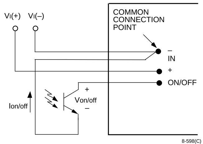
Figure 23. Remote On/Off Wiring Configuration
