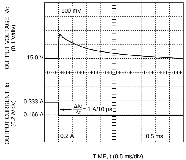
Figure 15. MW010C Typical Output Voltage Waveform for a Step Load Change from 50% to 25% of I_{o,max} ; V_i = 48 \text{ V} ; T_A = 25^\circ \text{C}
