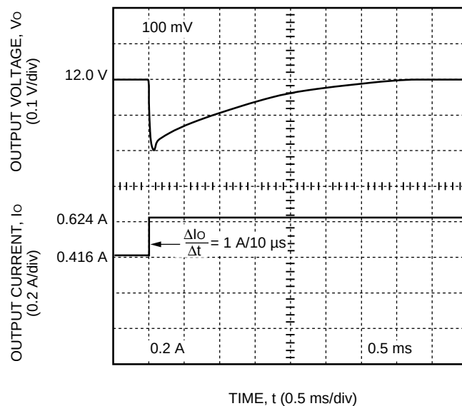
Figure 11. MW010B Typical Output Voltage Waveform for a Step Load Change from 50% to 75% of I_{o, \max} ; V_I = 48\text{ V} ; T_A = 25\text{ }^\circ\text{C}
