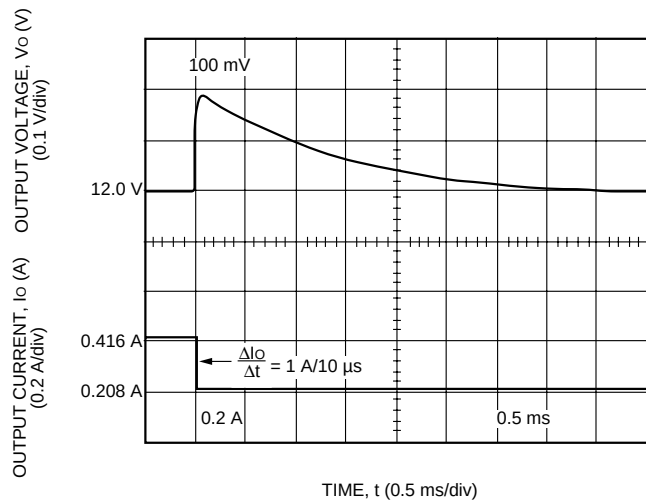
Figure 14. MW010B Typical Output Voltage Waveform for a Step Load Change from 50% to 25% of I_{o,max} ; V_i = 48 \text{ V} ; T_A = 25^\circ \text{C}
