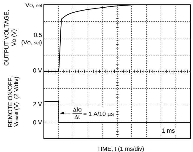
Figure 16. MW010A Typical Output Voltage Start-Up Waveform with Remote On/Off; I_o = 0.8 (I_{o,max}) ; V_i = 48 \text{ V} ; T_A = 25^\circ \text{C}
