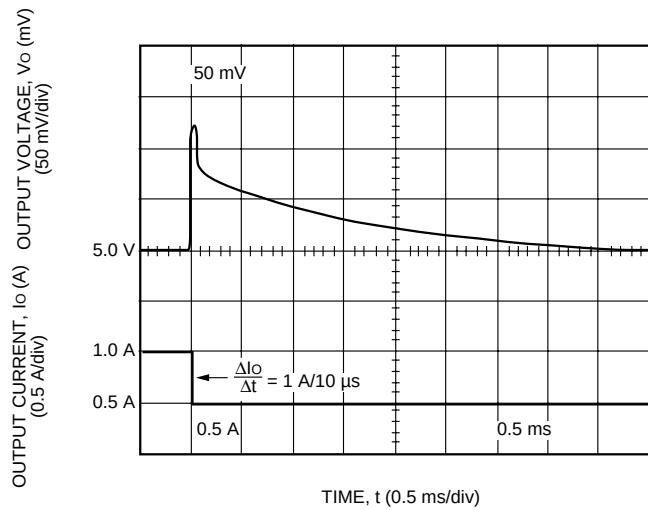
Figure 13. MW010A Typical Output Voltage Waveform for a Step Load Change from 50% to 25% of I_{o,max} ; V_i = 48 \text{ V} ; T_A = 25^\circ \text{C}
