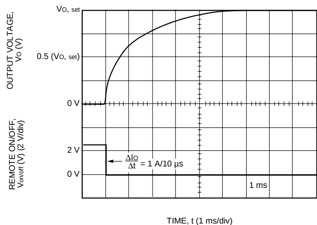
Figure 17. MW010B, C Typical Output Voltage Start-Up Waveform with Remote On/Off; I_o = 0.8 (I_{o, max}) ; V_i = 48 \text{ V} ; T_A = 25^\circ\text{C}
