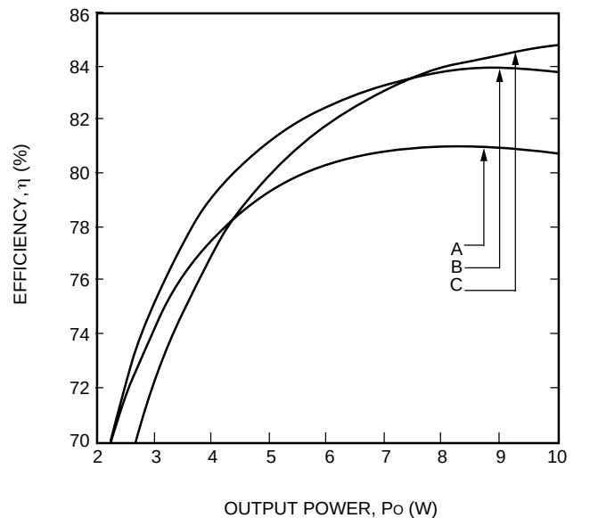
Figure 8. MW010A, B, C Typical Converter Efficiency as a Function of Output Power; V_i = 48\text{ V} ; T_A = 25\text{ }^{\circ}\text{C}
