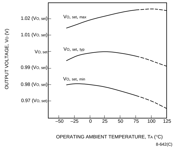
Figure 4. Typical Output Voltage Variation Over Operating Ambient Temperature Range; I_o = 0.8 (I_{o, \max}) ; V_i = 48 \text{ V}
