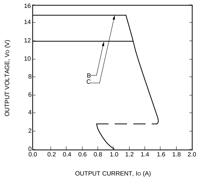
Figure 6. MW010B, C Typical Output Characteristic; V_i = 48\text{ V} ; T_A = 25\text{ }^{\circ}\text{C}
