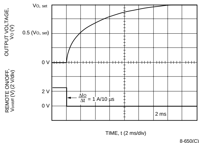
Figure 18. MW010BK, CL Typical Output Voltage Start-Up Waveform with Remote On/Off; I_o = 0.8 (I_{o, max}) ; V_i = 48 \text{ V} ; T_A = 25^\circ\text{C}
