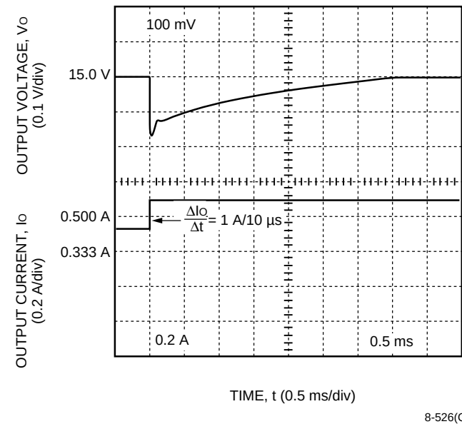
Figure 12. MW010C Typical Output Voltage Waveform for a Step Load Change from 50% to 75% of I_{o, \max} ; V_I = 48\text{ V} ; T_A = 25\text{ }^\circ\text{C}
