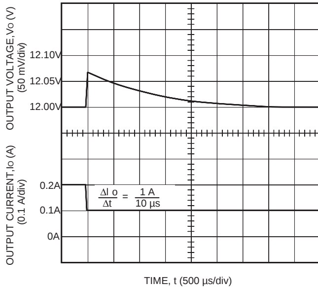
Figure 29. ME005B Typical Output Voltage Waveform for a Step Load Change from 50% to 25% of I_{o, max} with V_i = 48 V and T_A = 25 °C
