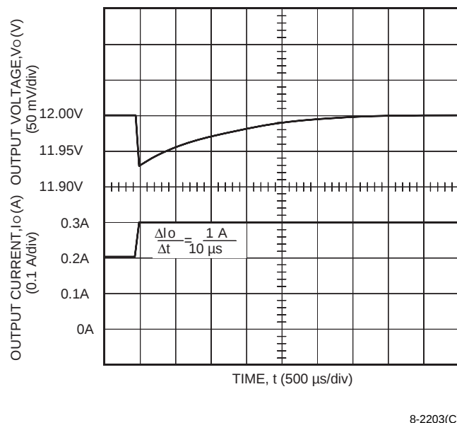
Figure 26. ME005B Typical Output Voltage Waveform for a Step Load Change from 50% to 75% of I_{o,max} with V_i = 48 V and T_A = 25 °C
