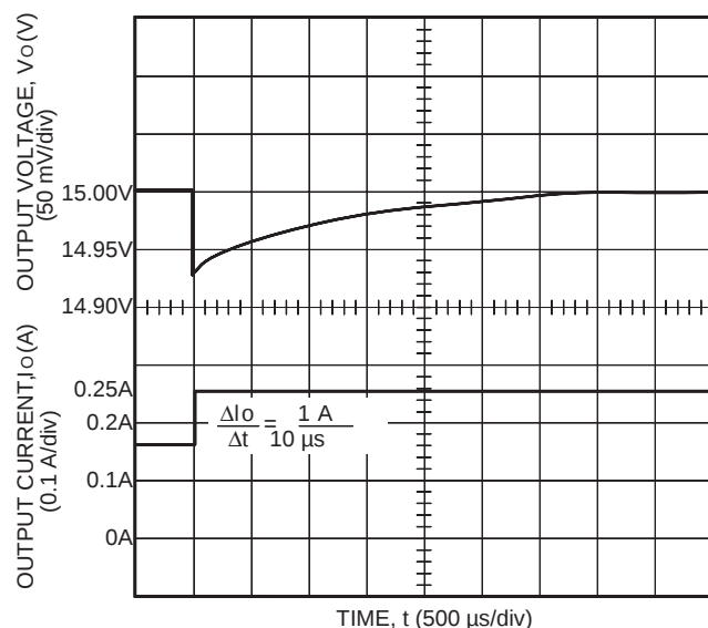
Figure 27. ME005C Typical Output Voltage Waveform for a Step Load Change from 50% to 75% of I_{o,max} with V_i = 48 V and T_A = 25 °C
