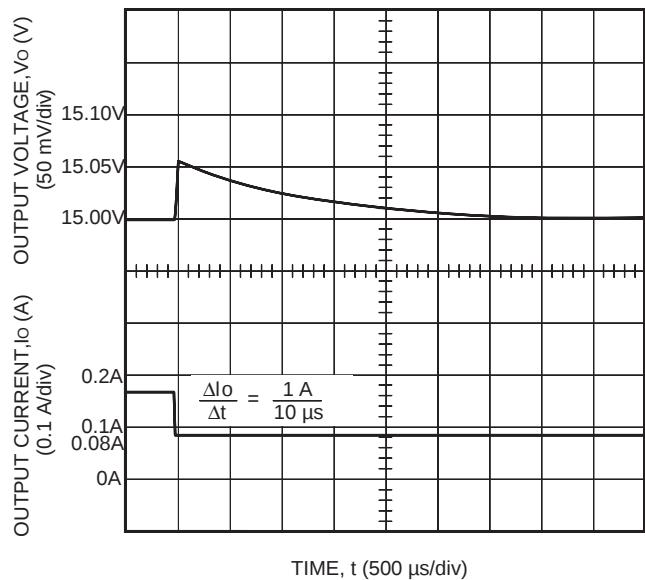
Figure 30. ME005C Typical Output Voltage Waveform for a Step Load Change from 50% to 25% of I_{o, max} with V_i = 48 V and T_A = 25 °C
