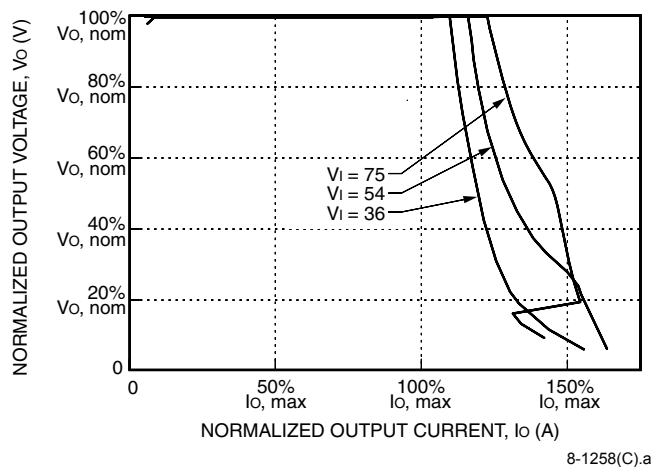
Figure 2. LW020A, B, C, F, and G Typical Output Characteristics, T_A = 25^\circ\text{C}
