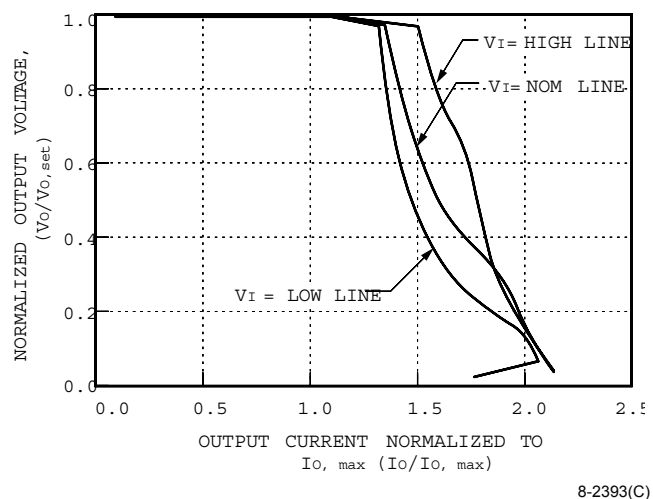
Figure 4. Lx005x Normalized Output Current vs. Normalized Output Voltage at T_c = 25\text{ }^{\circ}\text{C}
