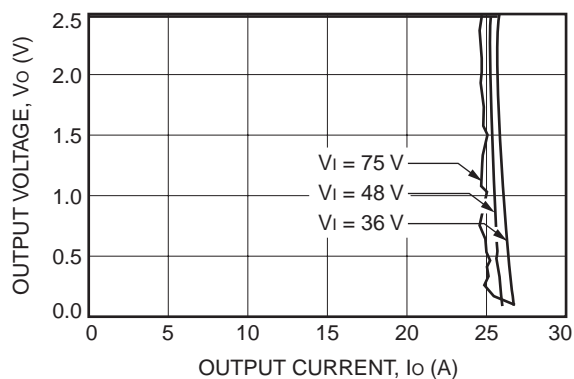
Figure 3. Typical JW100G Output Characteristics at Room Temperature
