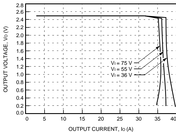
Figure 4. Typical JW150G Output Characteristics at Room Temperature
