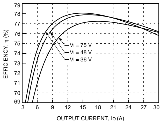
Figure 6. Typical JW150G Efficiency vs. Output Current at Room Temperature
