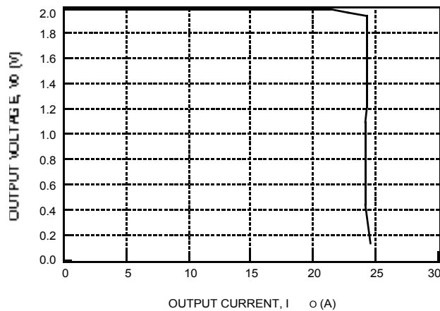
Figure 7. Typical JW100D Output Characteristics at Room Temperature
