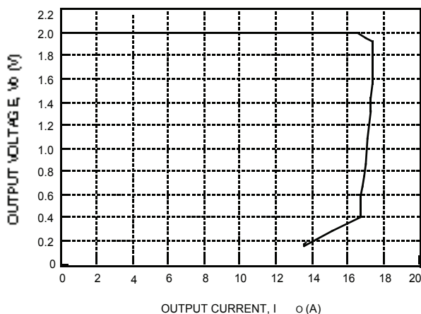
Figure 6. Typical JW075D Output Characteristics at Room Temperature
