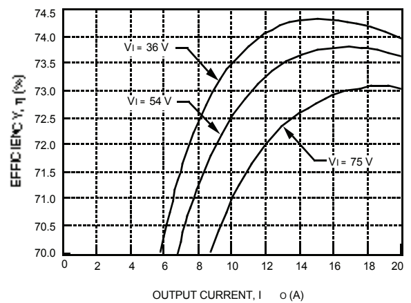
Figure 11. Typical JW100D Converter Efficiency vs. Output Current at Room Temperature
