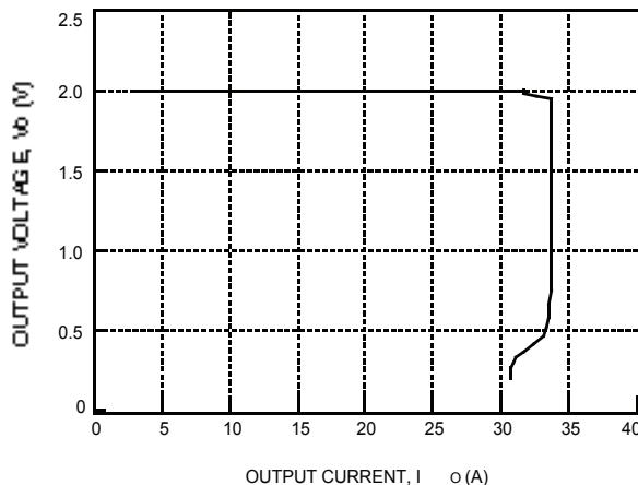
Figure 8. Typical JW150D Output Characteristics at Room Temperature
