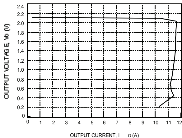
Figure 5. Typical JW050D Output Characteristics at Room Temperature
