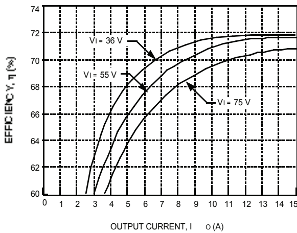
Figure 10. Typical JW075D Converter Efficiency vs. Output Current at Room Temperature
