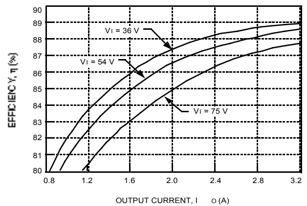
Figure 12. Typical JW075H Converter Efficiency vs. Output Current at Room Temperature
