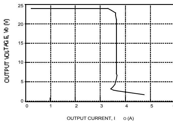
Figure 7. Typical JW075H Output Characteristics at Room Temperature
