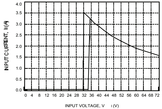
Figure 3. Typical JW100H Input Characteristics at Room Temperature
