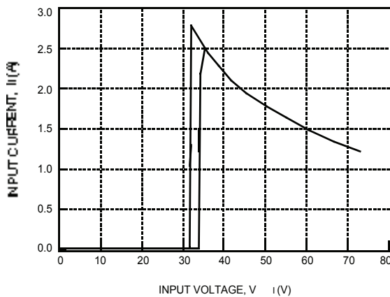
Figure 2. Typical JW075H Input Characteristics at Room Temperature
