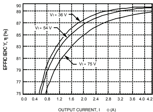
Figure 13. Typical JW100H Converter Efficiency vs. Output Current at Room Temperature
