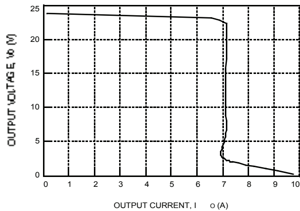
Figure 9. Typical JW150H Output Characteristics at Room Temperature
