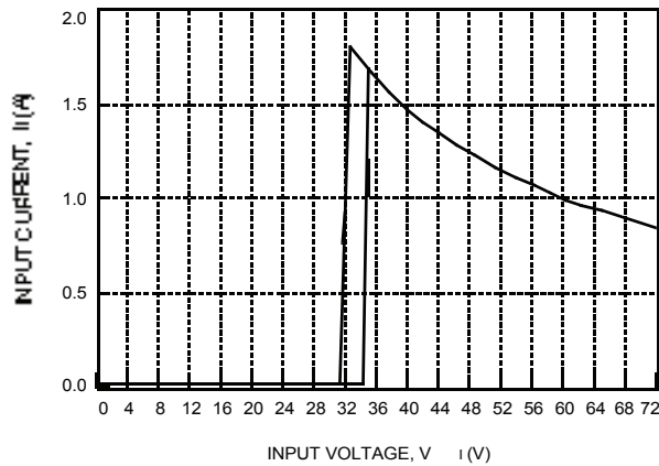
Figure 1. Typical JW050H Input Characteristics at Room Temperature
