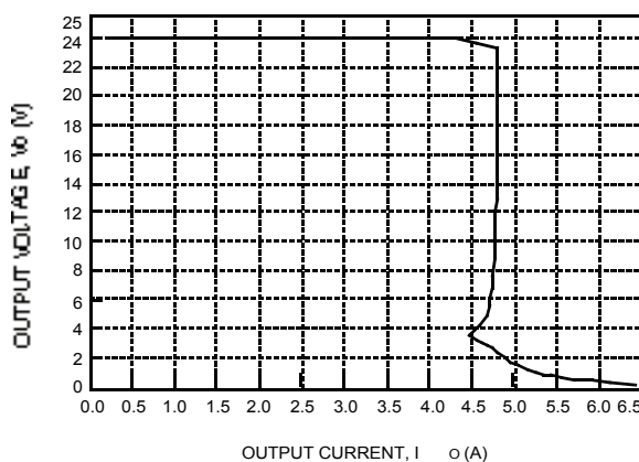
Figure 8. Typical JW100H Output Characteristics at Room Temperature
