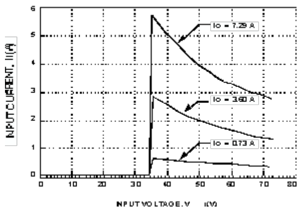
Figure 5. Typical JW175H Input Characteristics at Room Temperature
