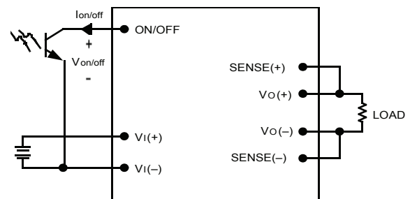
Figure 23. Remote On/Off Implementation 8-720 (C),c
