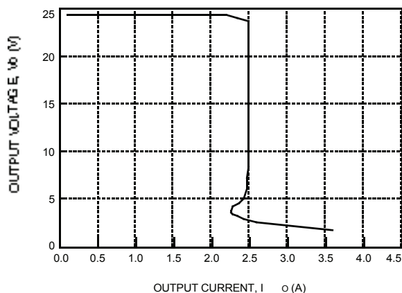
Figure 6. Typical JW050H Output Characteristics at Room Temperature
