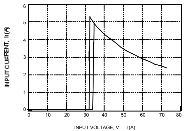
Figure 4. Typical JW150H Input Characteristics at Room Temperature
