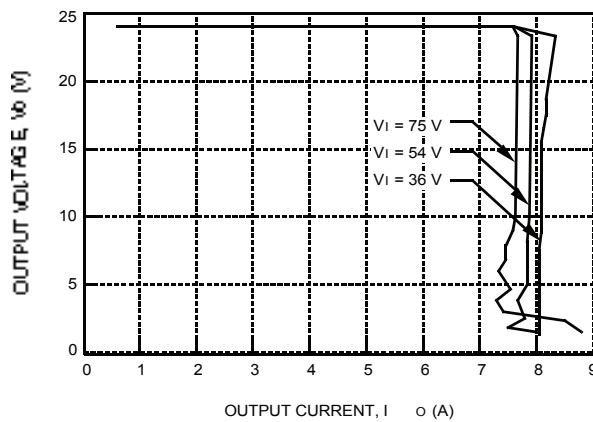
Figure 10. Typical JW175H Output Characteristics at Room Temperature
