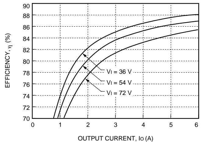
Figure 10. Typical JW075B Converter Efficiency vs. Output Current at Room Temperature
