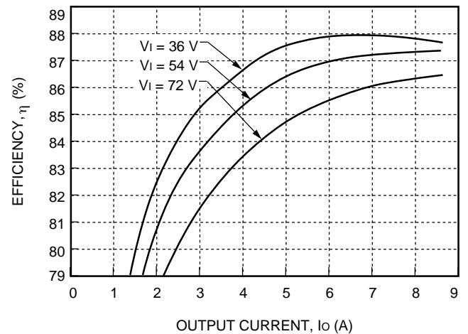
Figure 11. Typical JW100B Converter Efficiency vs. Output Current at Room Temperature
