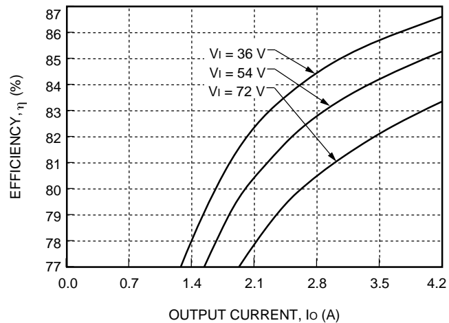
Figure 9. Typical JW050B Converter Efficiency vs. Output Current at Room Temperature
