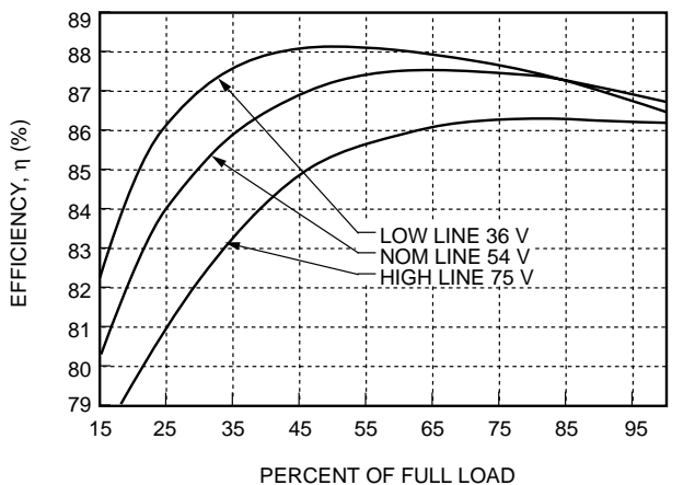
Figure 6. Typical JW060ABK Converter Efficiency vs. Output Current at Room Temperature
