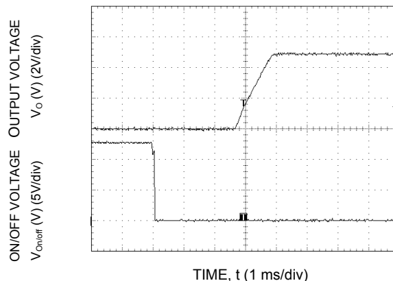
Figure 10. Typical Start-Up Characteristics from Remote ON/OFF.
