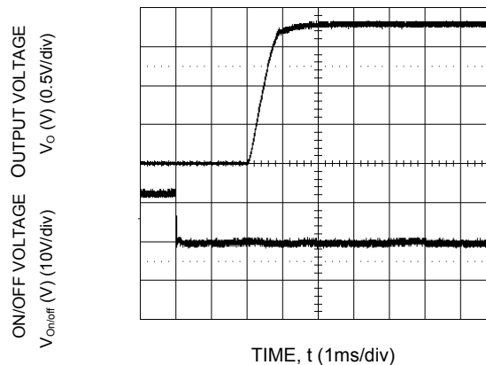
Figure 28. Typical Start-Up Characteristics from Remote ON/OFF.
