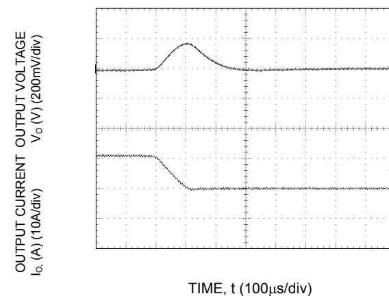
Figure 11. Transient Response to Dynamic Load Change from 50% to 25% of full load current.
