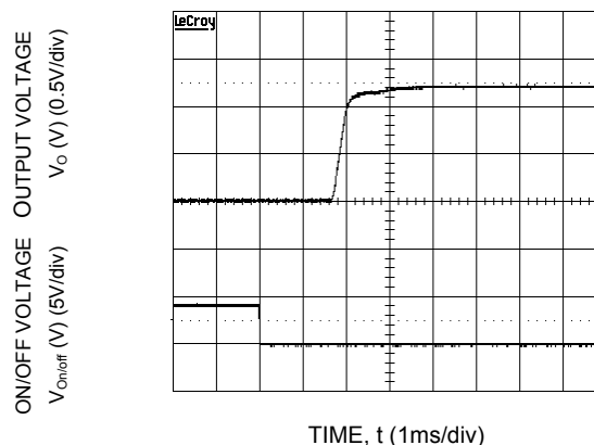
Figure 40. Typical Start-Up Characteristics from Remote ON/OFF.
