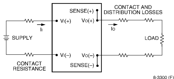
Figure 44. Output Ripple and Noise Test Setup.
