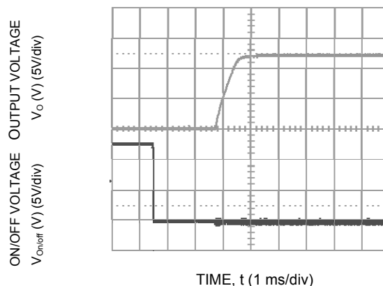
Figure 4. Typical Start-Up Characteristics from Remote ON/OFF.
