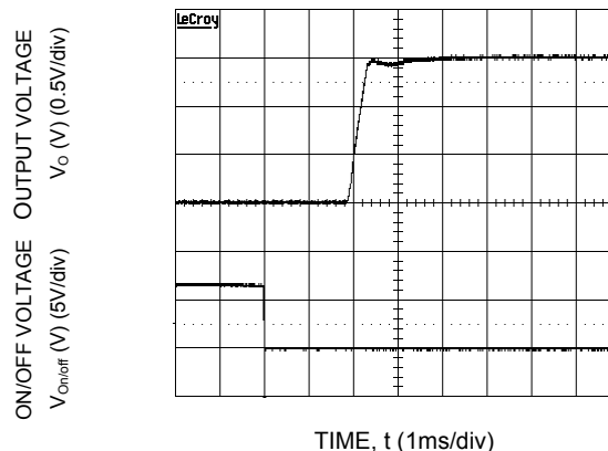
Figure 34. Typical Start-Up Characteristics from Remote ON/OFF.
