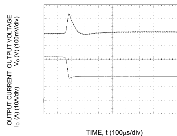
Figure 23. Transient Response to Dynamic Load Change from 50% to 25% of full load current.
