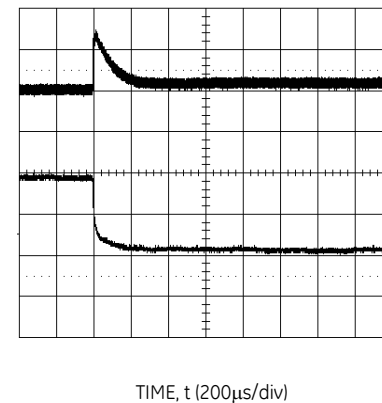
Figure 41. Transient Response to Dynamic Load Change from 50% to 25% of full load current.
