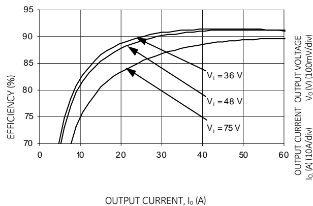
Figure 14. Converter Efficiency Vs Load at Room temperature.
