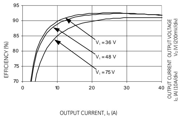
Figure 8. Converter Efficiency Vs Load at Room temperature.
