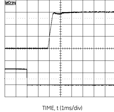
Figure 34. Typical Start-Up Characteristics from Remote ON/OFF.
