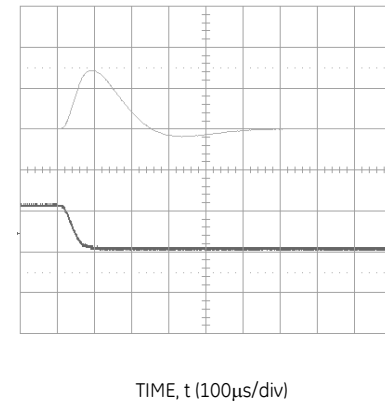
Figure 5. Transient Response to Dynamic Load Change from 50% to 25% of full load current.
