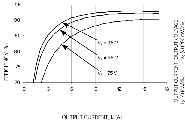
Figure 2. Converter Efficiency Vs Load at Room temperature.
