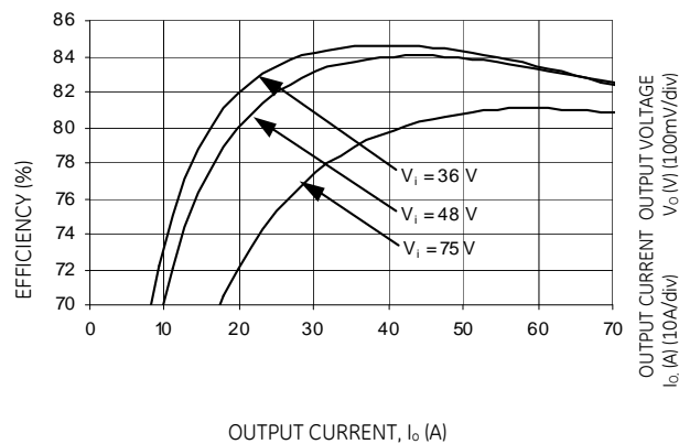
Figure 38. Converter Efficiency Vs Load at Room temperature.
