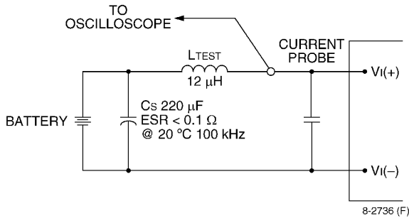
Figure 43. Input Reflected Ripple Current Test Setup.
