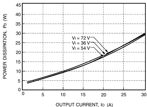
Figure 32. JFW150A Power Dissipation vs. Output Current at 25 °C
