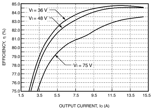
Figure 10. Typical JFW075A Converter Efficiency vs. Output Current at Room Temperature
